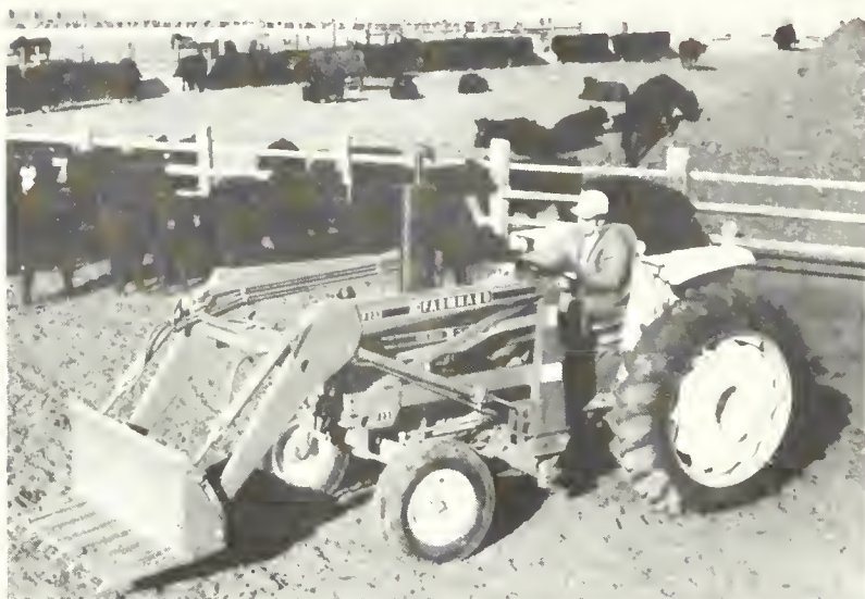
Figure 2.4.19 Typical front-mounted silage or manure fork. Power is supplied by the tractor hydraulics or an auxiliary hydraulic pump. Courtesy: Farmhand Inc., Hopkins, Minn.
