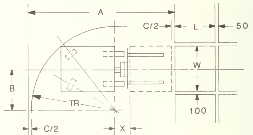
Figure 2.4.1 Aisle width allowance for fork trucks. Dimensions are in millimeters.
