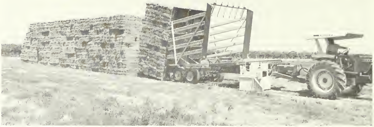
Figure 2.4.37 Pull-type bale wagon unloading at a 9 bale high stack. Courtesy: Sperry New Holland, New Holland, Pa.
